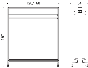
QCHA.125/165 | Coat hanger
