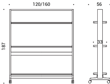
QCB.125/165 | Coffee station
