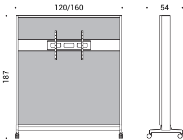
QMSA.125/165 | Monitor stand with back panel
