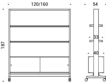
QSE.125/165 | Space divider
