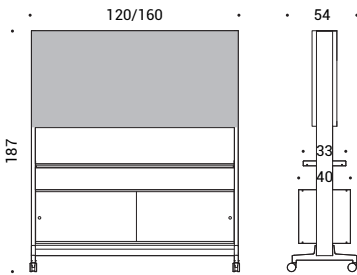
QSD.125/165 | Space divider
