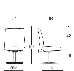
4-spoke swivel base and RIV armrests - Executive
